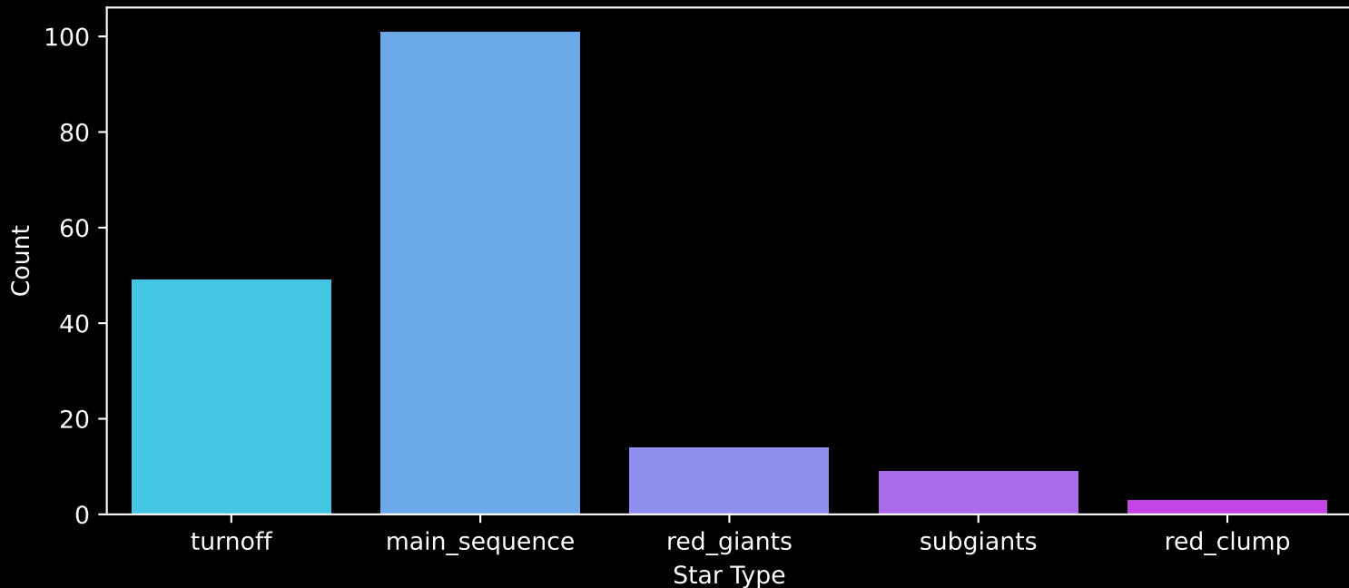
APOGEE DR17 Field: [174+49_MGA] Count plot of Star Type
