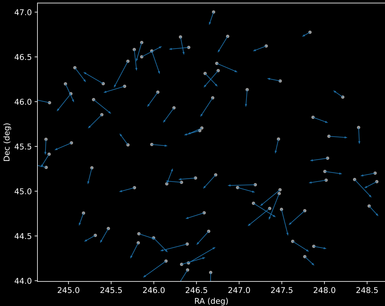
APOGEE DR17 Cluster 0 Proper Motion Vectors (n=78)
