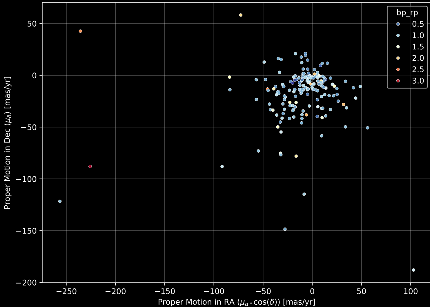
APOGEE DR17 Field: [174+49_MGA] Proper Motion Diagram (n= 176)
