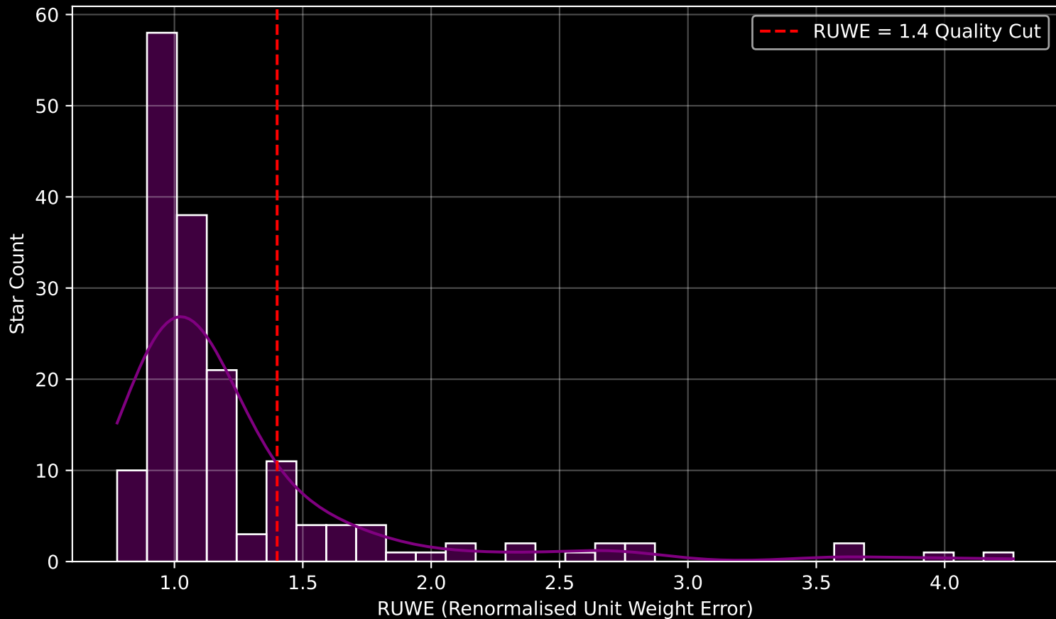
GAPOGEE DR17 Field [174+49_MGA] RUWE Distribution (n= 168)
