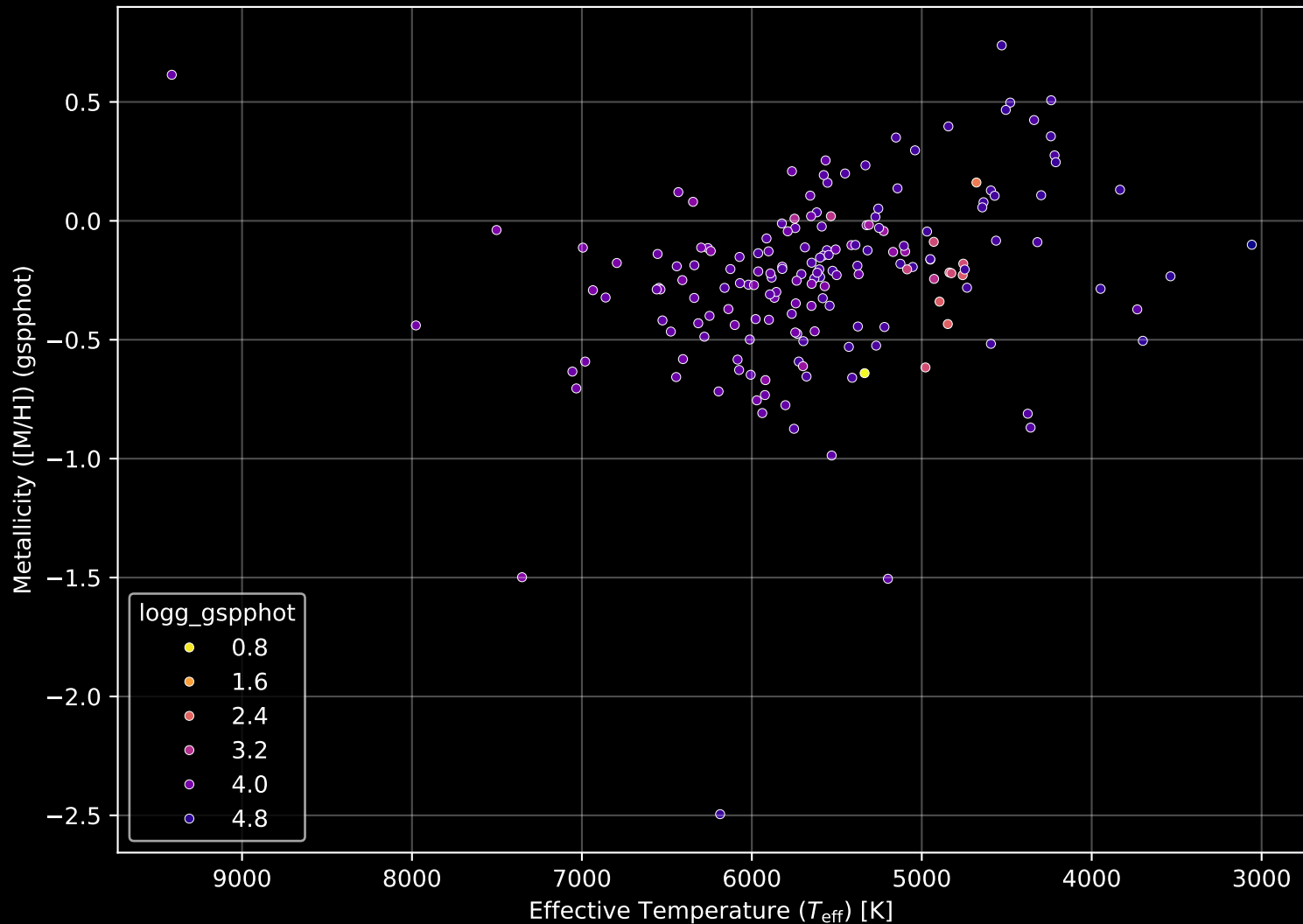
APOGEE DR17 Field: [174+49_MGA] Stellar Population Parameters (n= 176)
