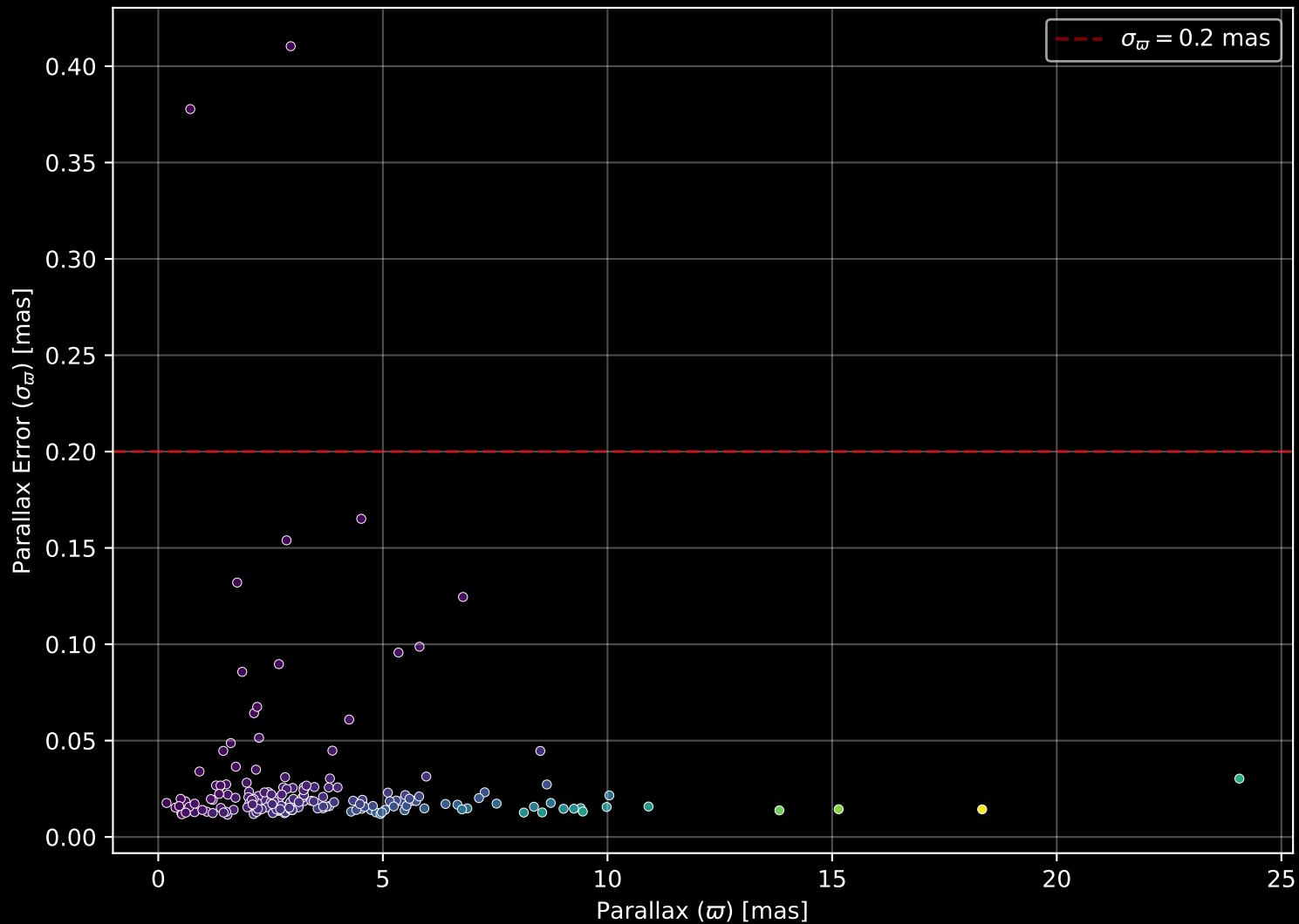
APOGEE DR17 Field: [174+49_MGA] Parallax Quality (n= 176)
