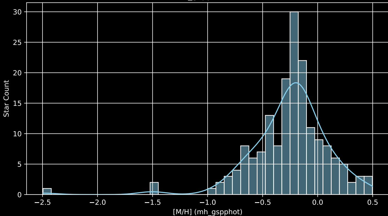
APOGEE DR17 Field: [174+49_MGA [M/H] (mh_gspphot) (n= 173)
